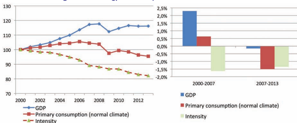
Figure 2: Energy consumption and GDP in the EU 6
