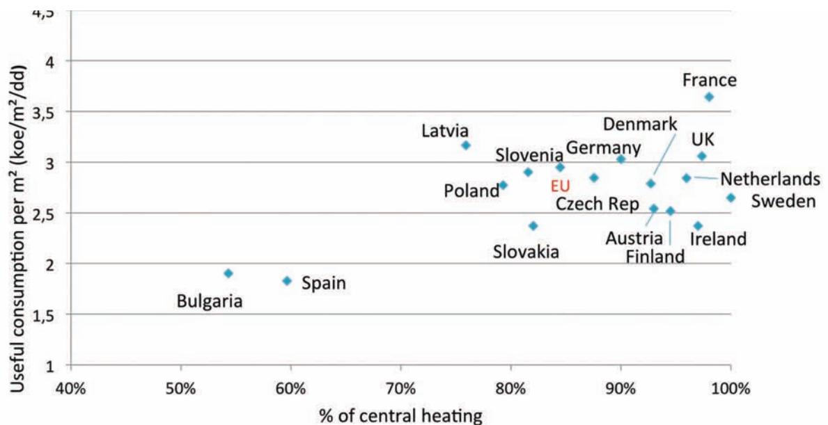
Figure 47: Energy use for space heating per m 2 and degree day (2012) 36
