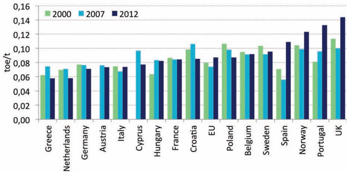
Figure 20: Trends in the specific consumption of cement in EU countries
