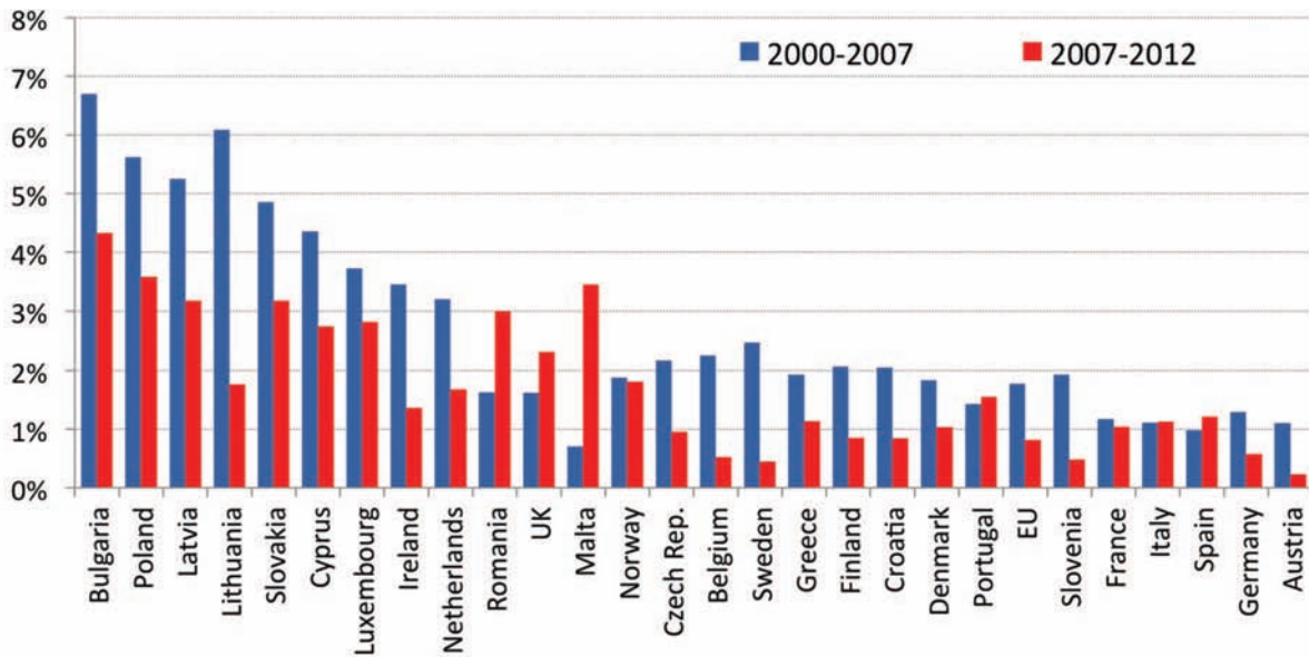
Figure 25: Energy efficiency trends in industry in EU countries (%/year)
