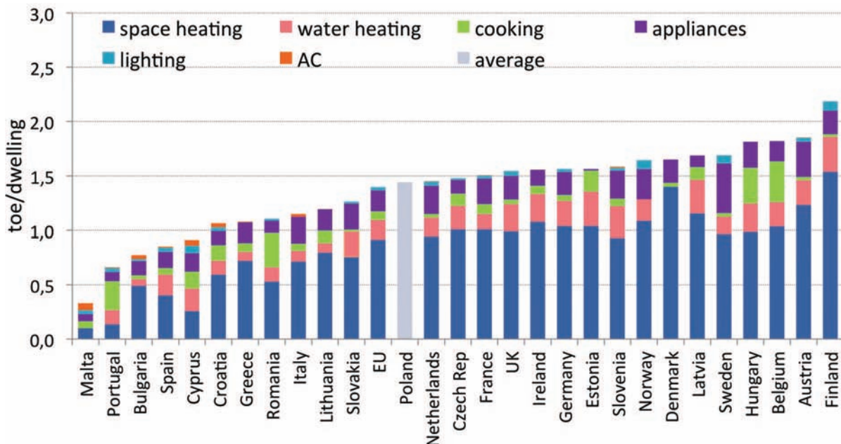
Figure 42: Breakdown of household energy use by end-use (2012)
