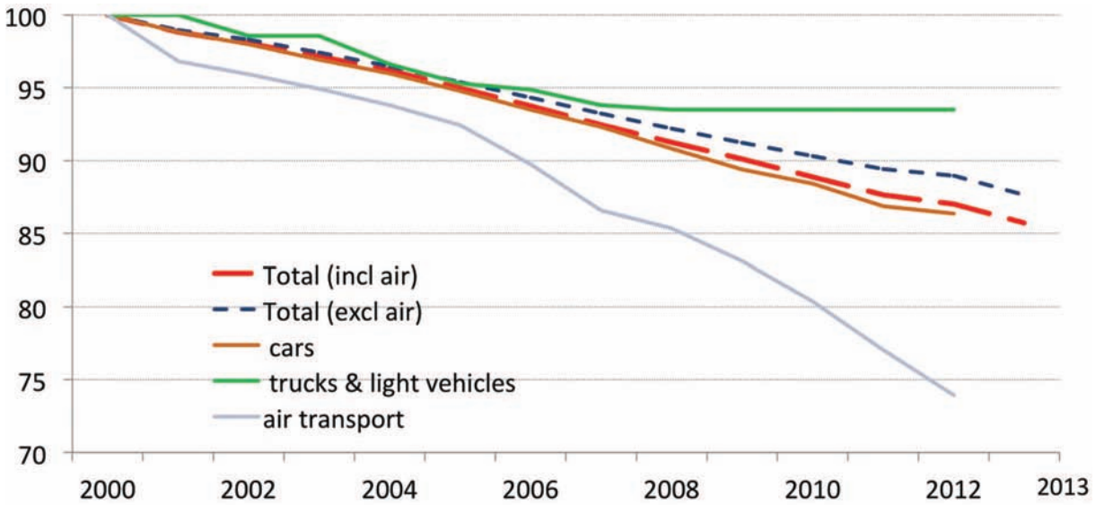
Figure 36: Energy efficiency progress in transport in the EU
