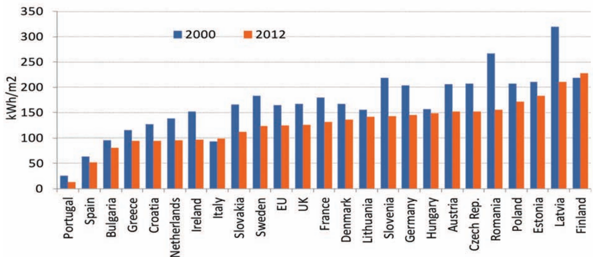
Figure 45: Energy use for space heating per m 2 33
