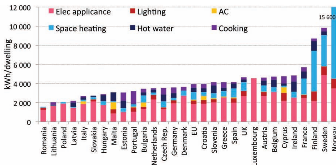
Figure 43: Average electricity consumption per dwelling (2012)
