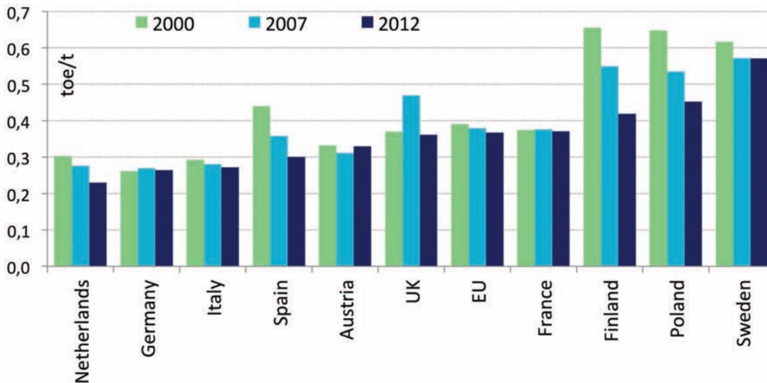
Figure 22: Trends in the energy consumption per tonne of paper 24
