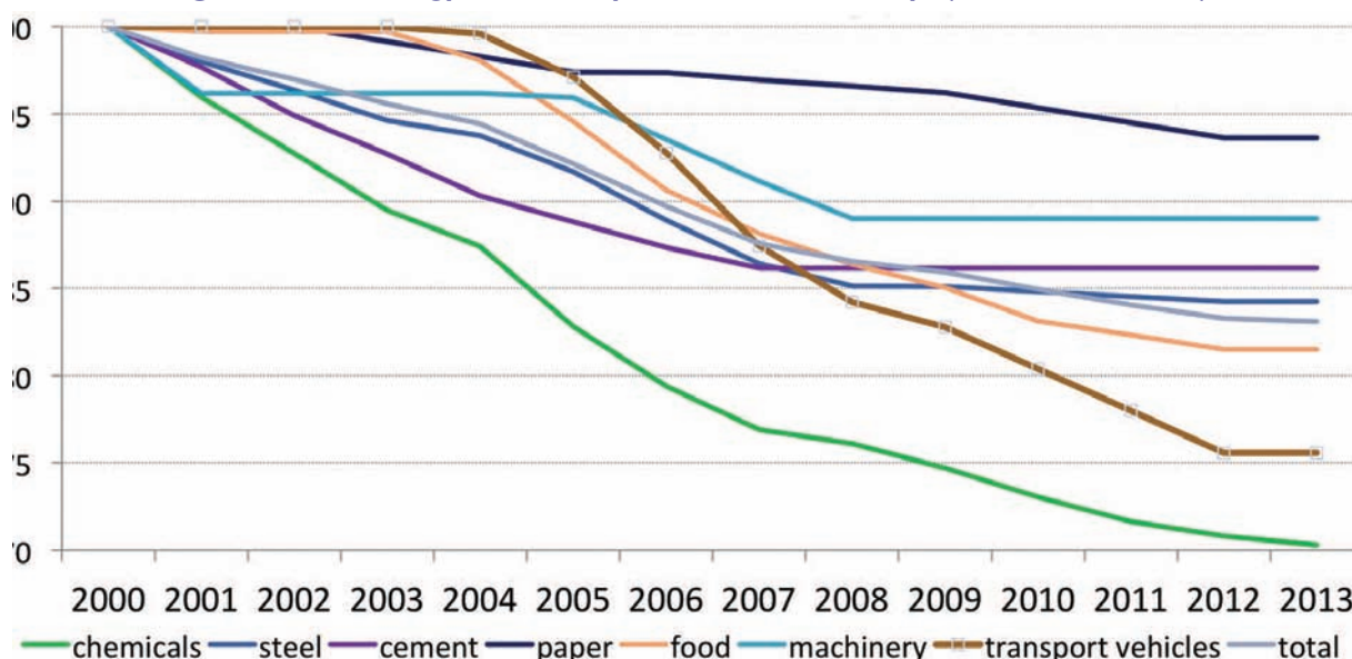
Figure 24: Energy efficiency index in industry (EU, 2000-2013)
