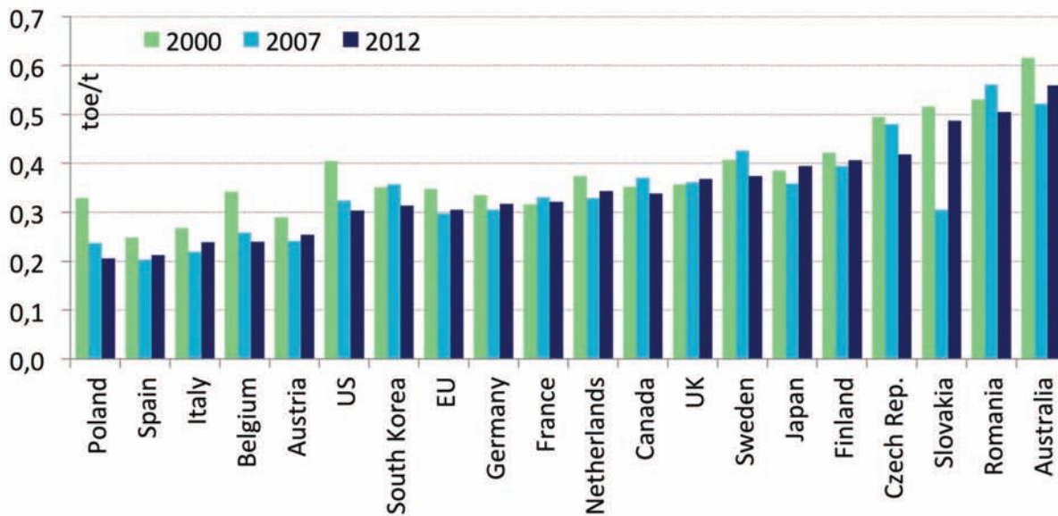
Figure 19: Specific energy consumption per tonne of steel 22
