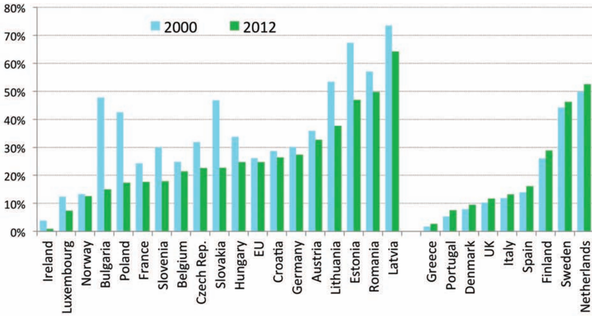
Figure 39: Share of rail and water in total freight traffic
