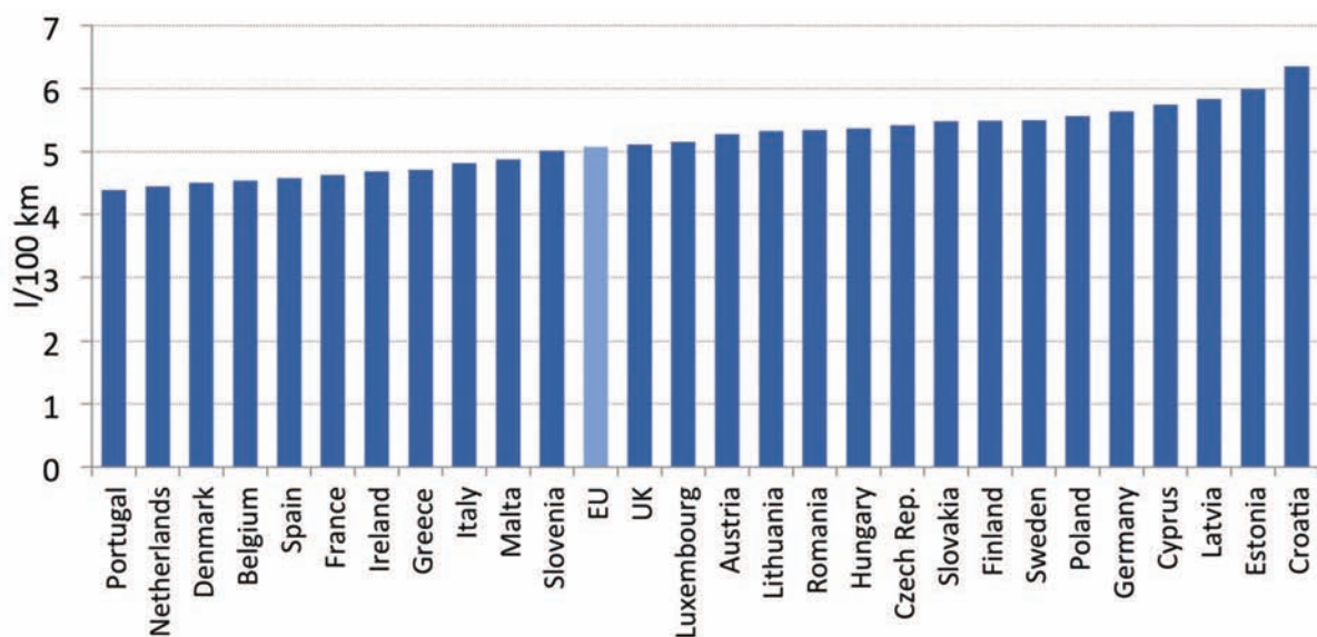
Figure 32: Specific consumption of new cars in the EU (2013)
