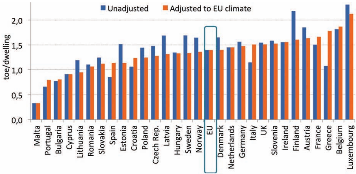
Figure 44: Household energy consumption per dwelling (2012)
