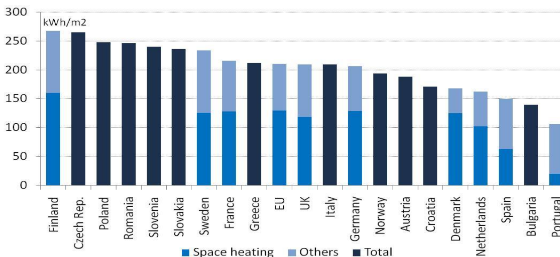
Figure 5: Energy consumption in building (kWh/m 2 ) in 2012
