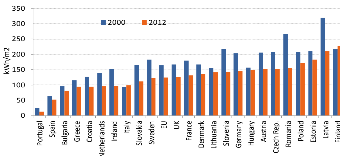
Figure 14: Energy use for space heating per \text{m}^2
