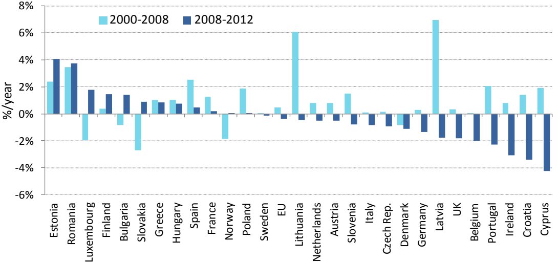
Figure 9: Trends in electricity consumption per dwelling
